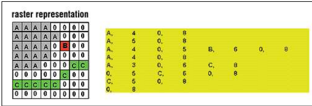
Figure 10. Run-length encoding
